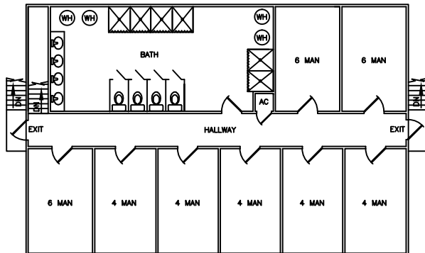
UPPER LEVEL NOT TO SCALE
