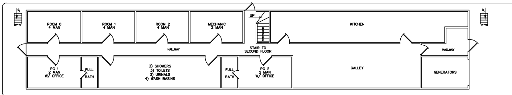
LOWER LEVEL NOT TO SCALE QUARTERS BARGE 'MINDY'
